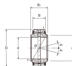
GE・ES-2RS
